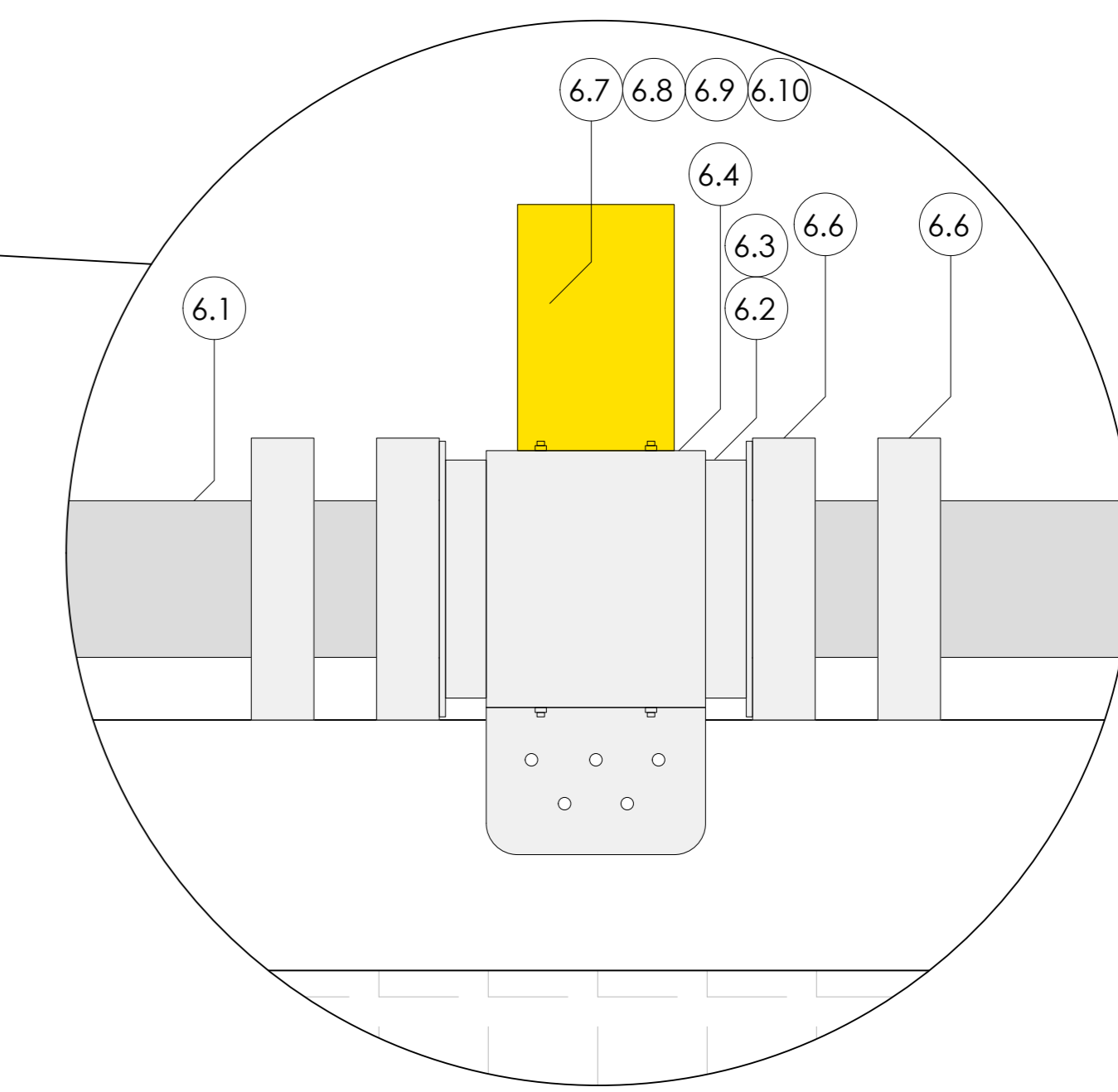
Rotation part Scale 1:10
