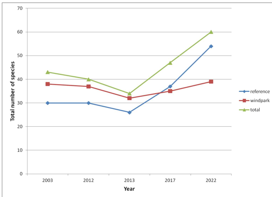
Figure 4-18: Total number of species within the windpark (red line) and in the reference locations (blue line) and in total (green line).
