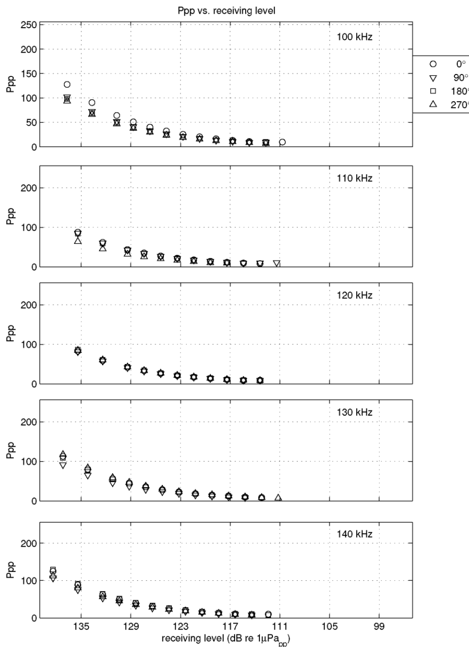
Figure II-14 Calibration results: Ppp vs frequency (this page) and Ppp vs receiving levels (next page) CPOD 1861 after deployment.
