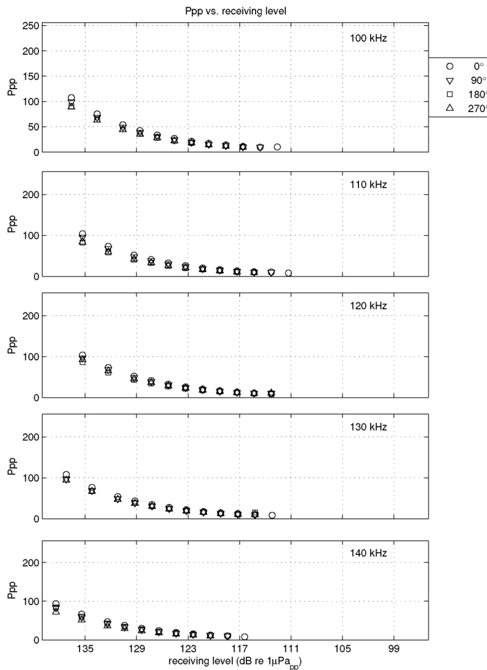
Figure II-23 Calibration results: Ppp vs frequency (this page) and Ppp vs receiving levels (next page) CPOD 3174 after deployment.
