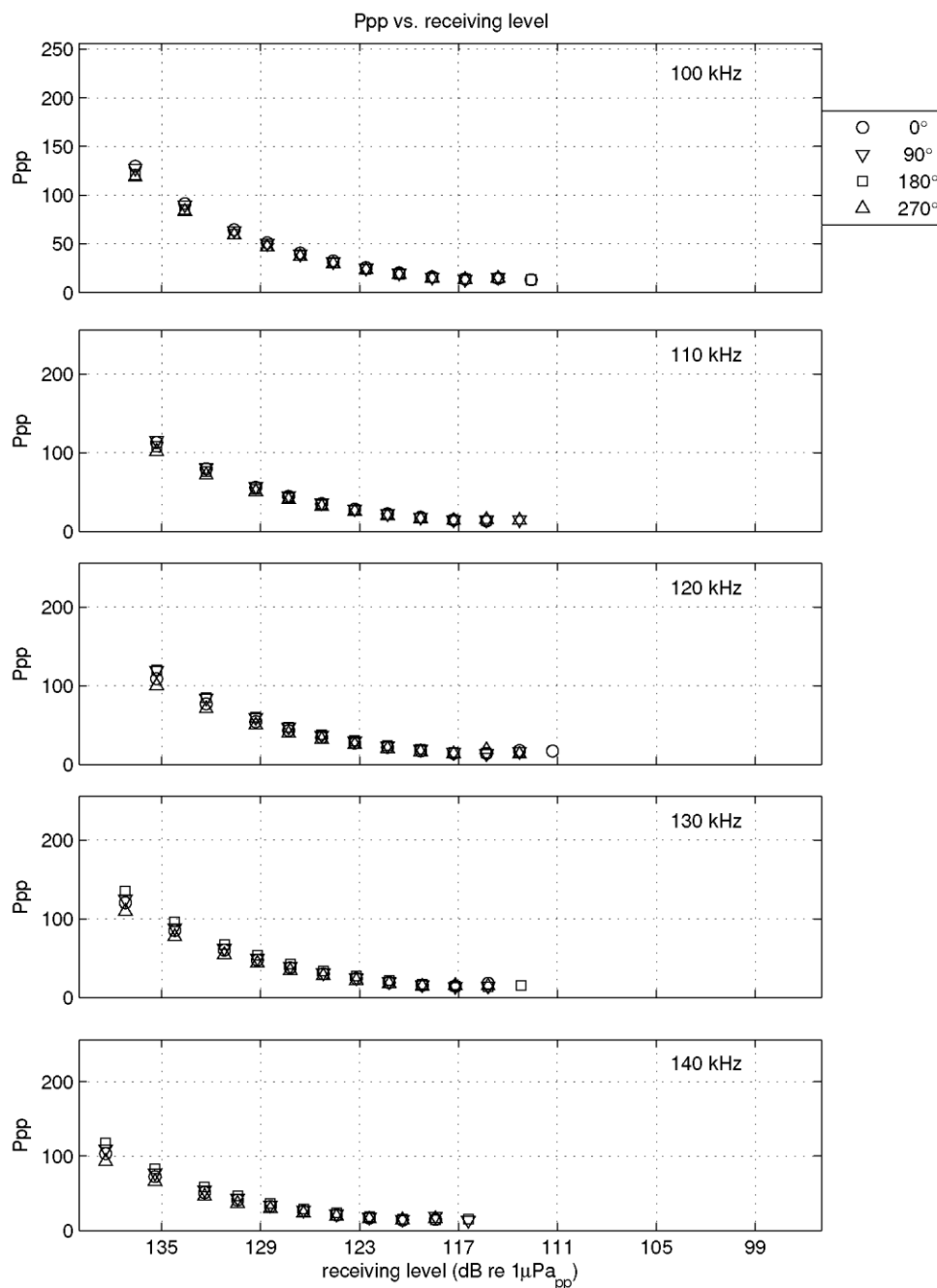
Figure II-4 Calibration results: Ppp vs frequency (this page) and Ppp vs receiving levels (next page) CPOD 395 after deployment.
