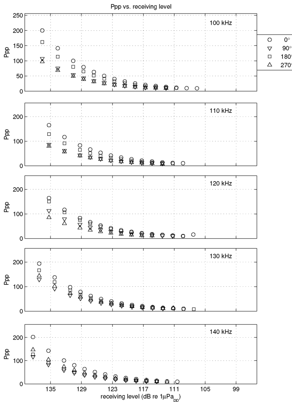
Figure II-9 Calibration results: Ppp vs frequency (this page) and Ppp vs receiving levels (next page) CPOD 1746 after deployment.
