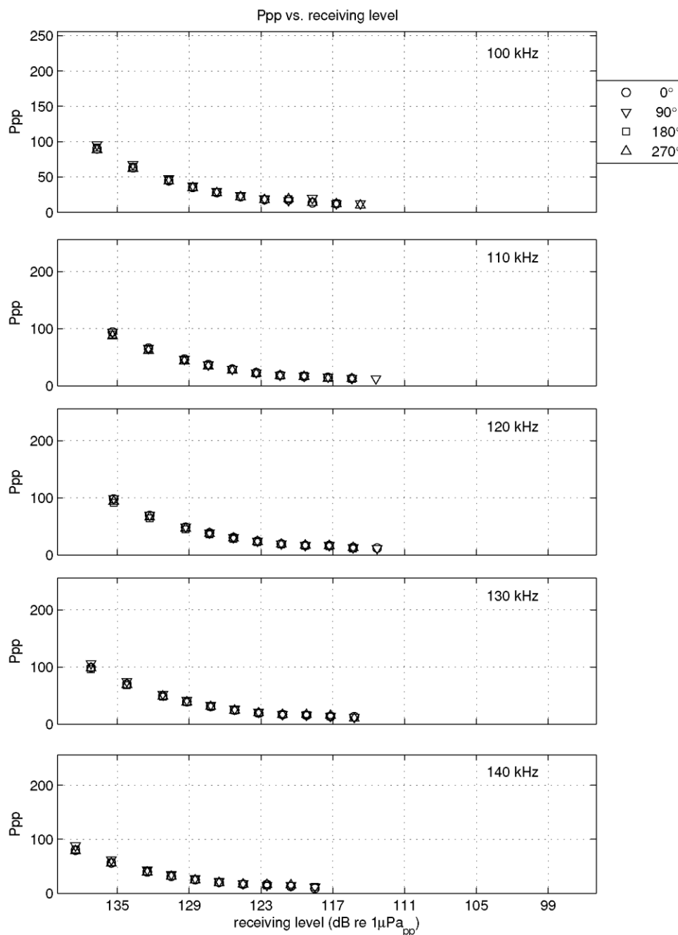
Figure II-22 Calibration results: Ppp vs frequency (this page) and Ppp vs receiving levels (next page) CPOD 3173 after deployment.
