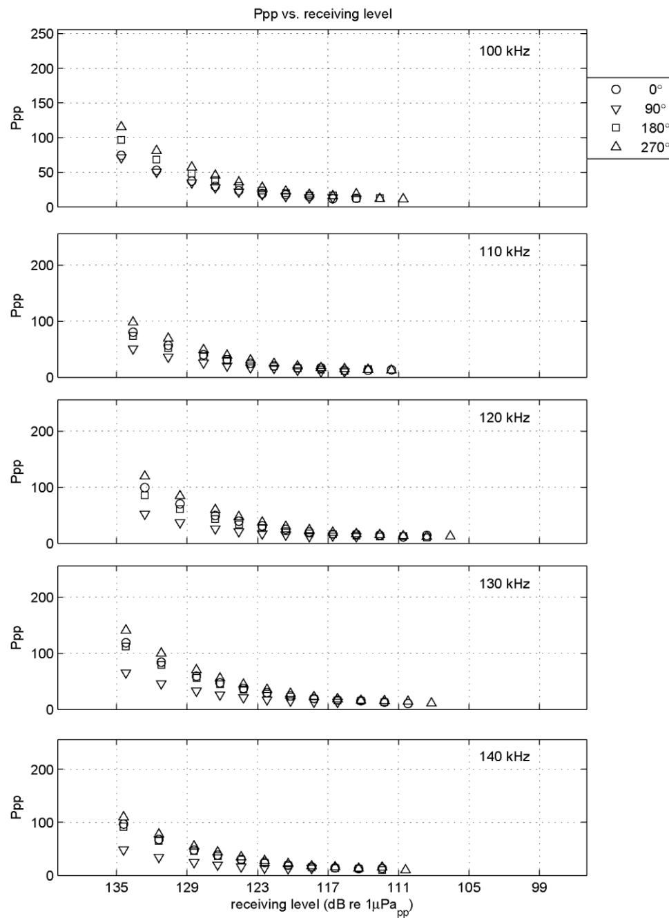
Figure I-7 Calibration results: Ppp vs frequency (this page) and Ppp vs receiving levels (next page) CPOD 1519 before deployment.
