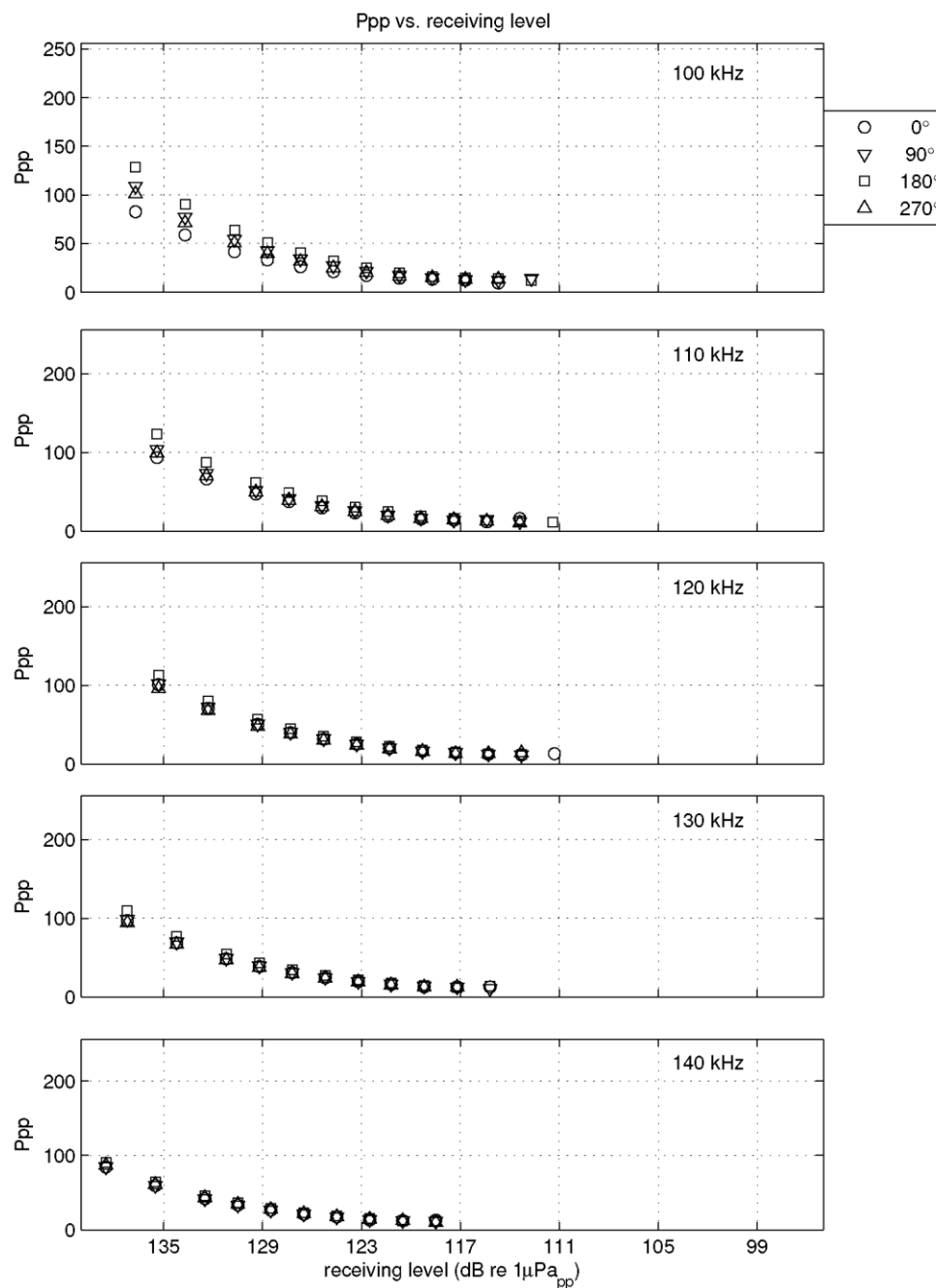
Figure II-24 Calibration results: Ppp vs frequency (this page) and Ppp vs receiving levels (next page) CPOD 3177 after deployment.
