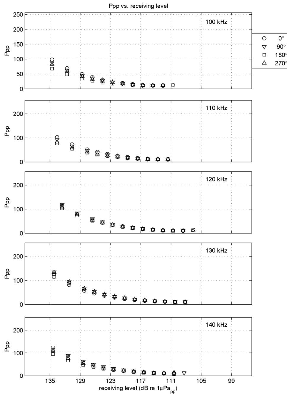
Figure I-8 Calibration results: Ppp vs frequency (this page) and Ppp vs receiving levels (next page) CPOD 1747 before deployment.
