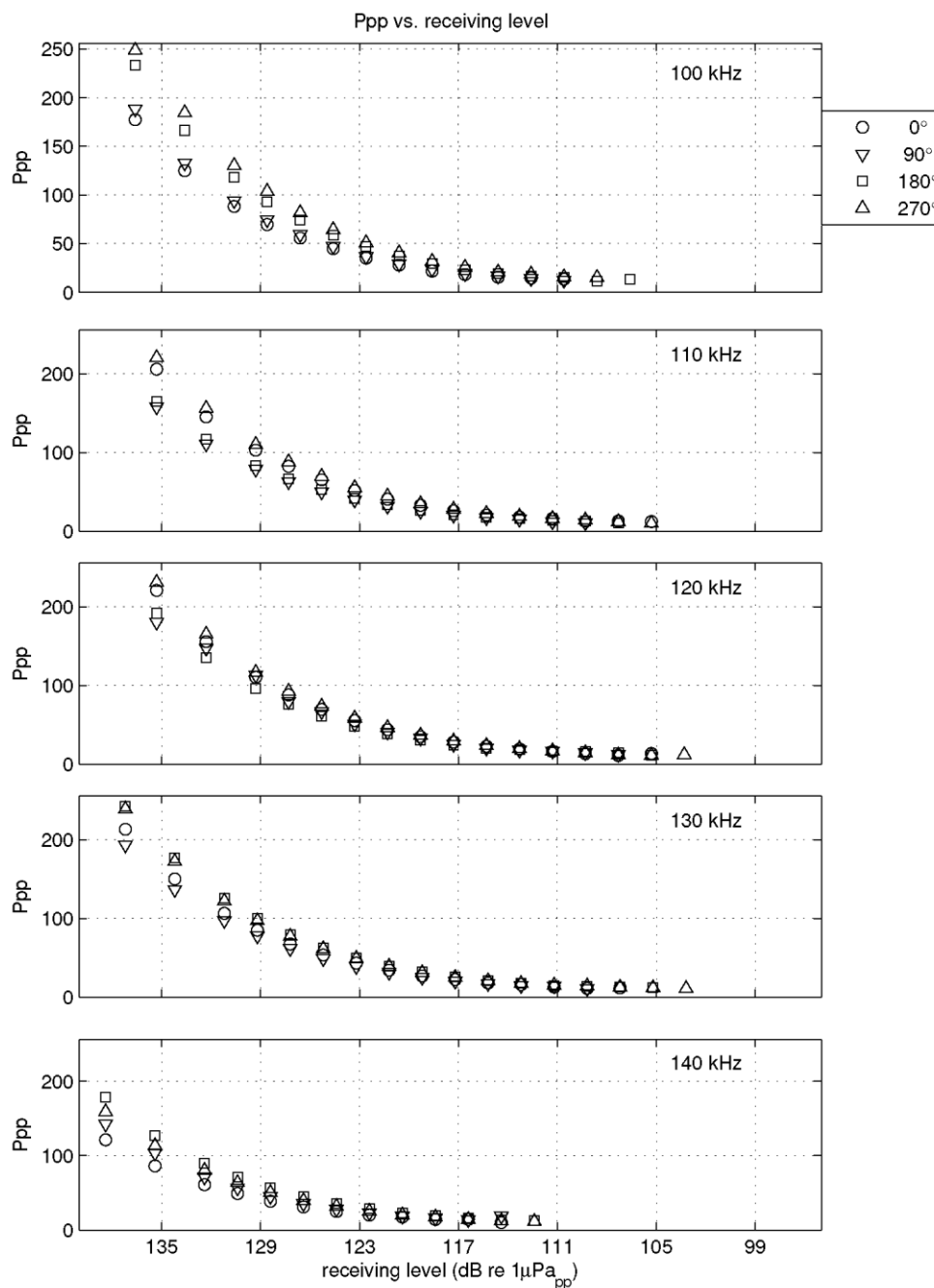
Figure II-7 Calibration results: Ppp vs frequency (this page) and Ppp vs receiving levels (next page) CPOD 1519 after deployment.
