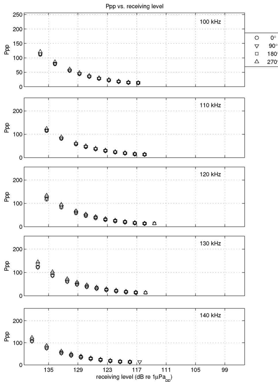
Figure II-3 Calibration results: Ppp vs frequency (this page) and Ppp vs receiving levels (next page) CPOD 394 after deployment.
