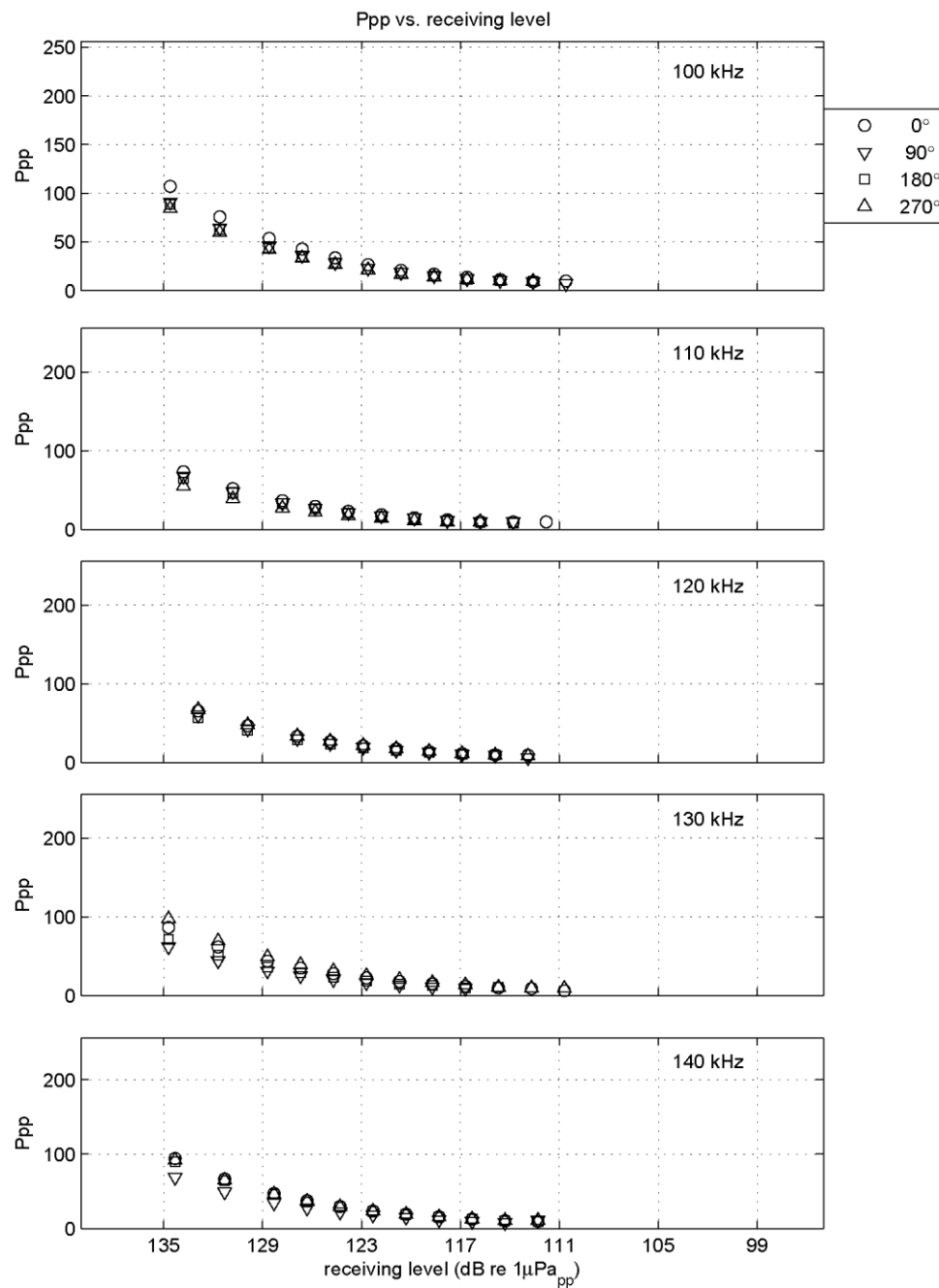
Figure I-12 Calibration results: Ppp vs frequency (this page) and Ppp vs receiving levels (next page) CPOD 1861 before deployment.
