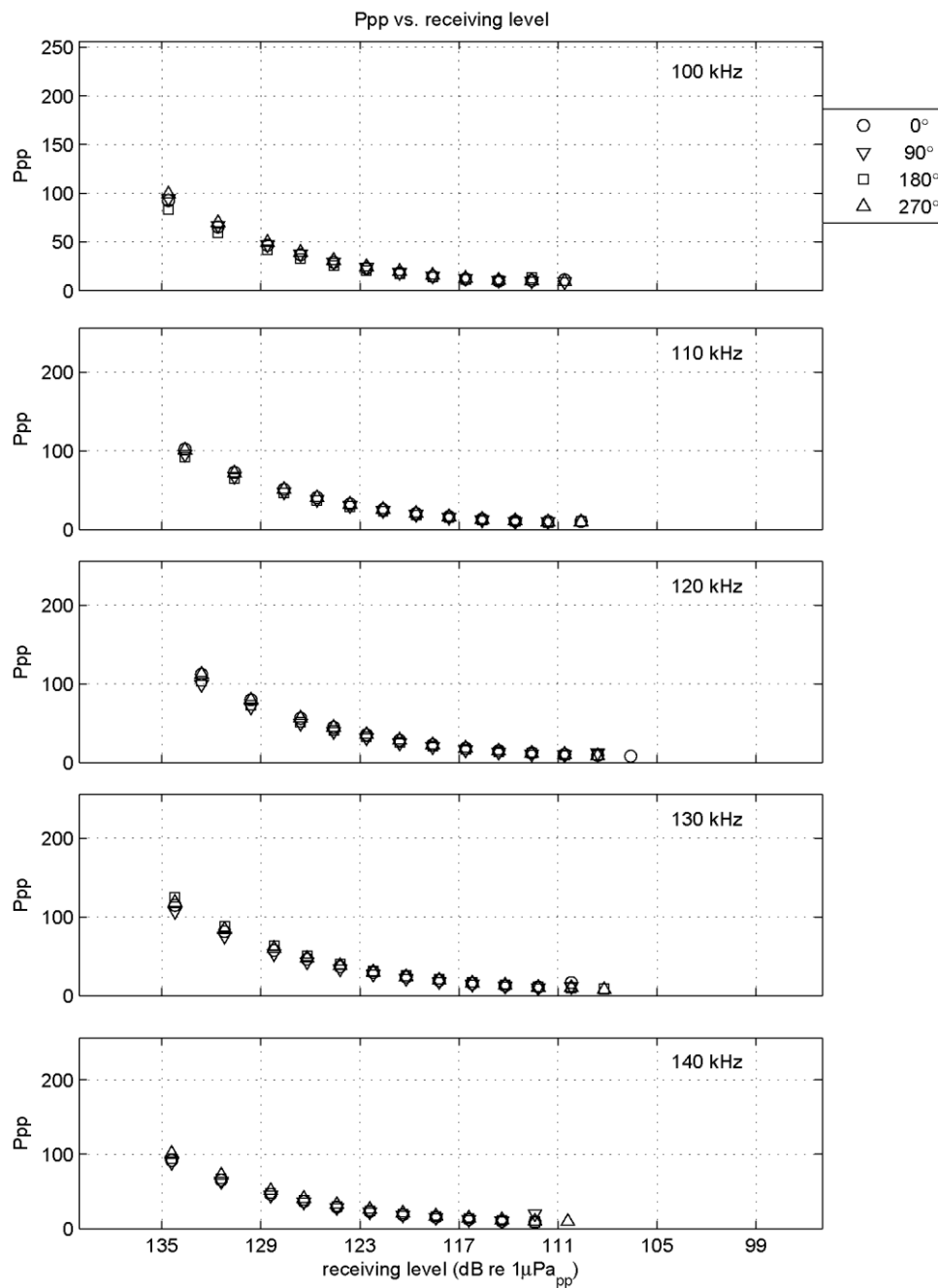
Figure I-17 Calibration results: Ppp vs frequency (this page) and Ppp vs receiving levels (next page) CPOD 1884 before deployment.
