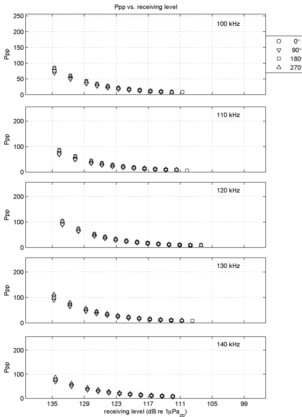
Figure I-5 Calibration results: Ppp vs frequency (this page) and Ppp vs receiving levels (next page) CPOD 862 before deployment.
