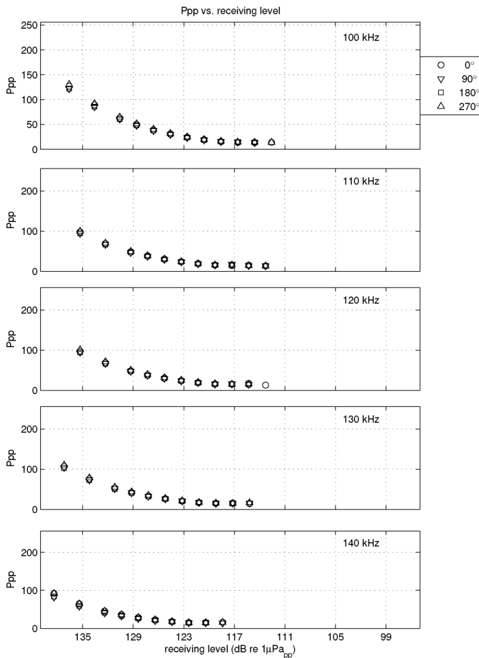
Figure II-2 Calibration results: Ppp vs frequency (this page) and Ppp vs receiving levels (next page) CPOD 392 after deployment.
