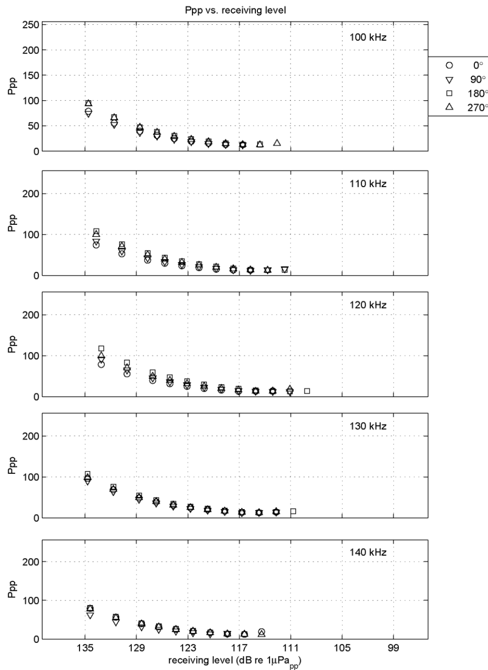
Figure I-11 Calibration results: Ppp vs frequency (this page) and Ppp vs receiving levels (next page) CPOD 1859 before deployment.
