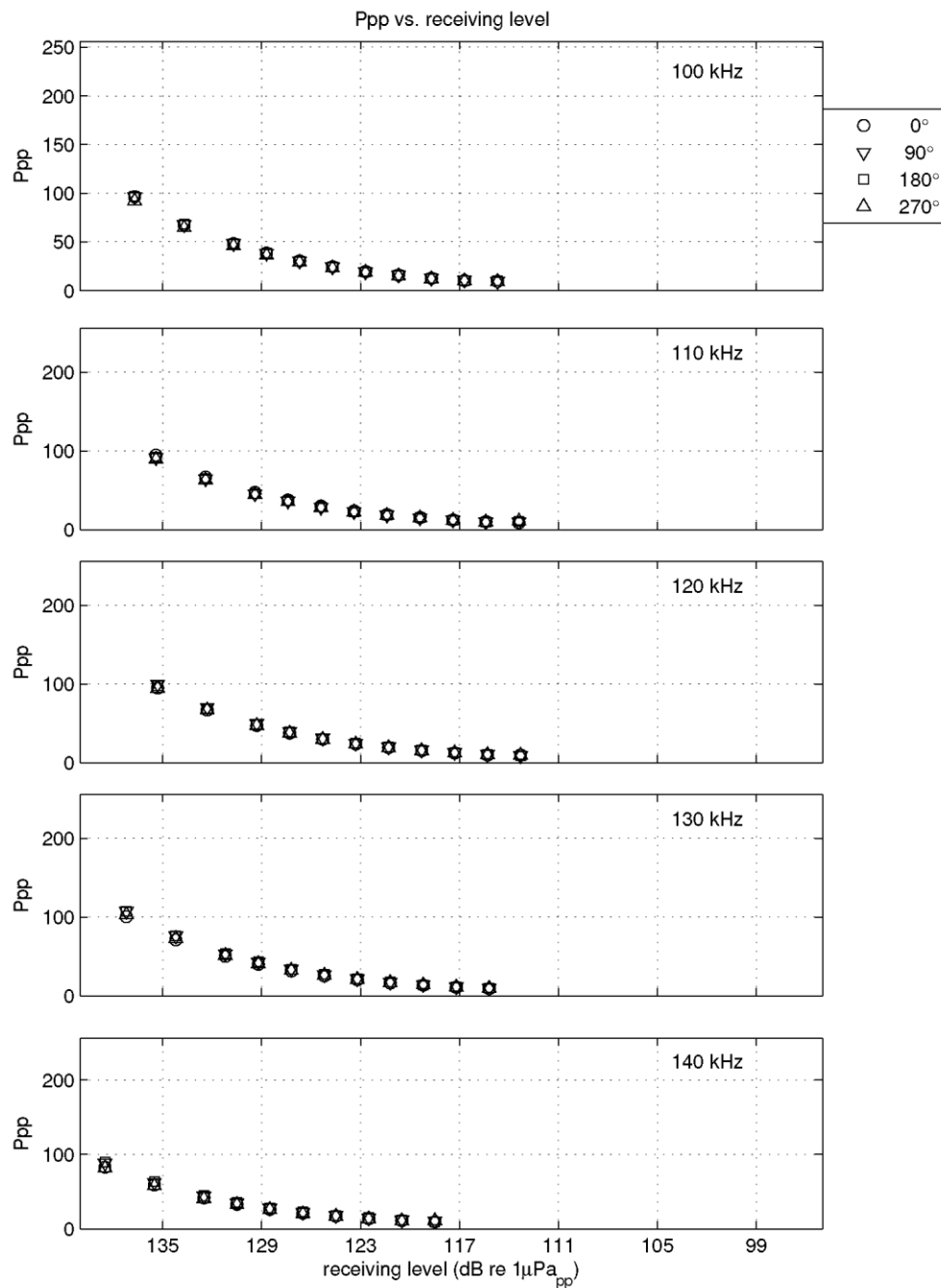
Figure II-20 Calibration results: Ppp vs frequency (this page) and Ppp vs receiving levels (next page) CPOD 3160 after deployment.
