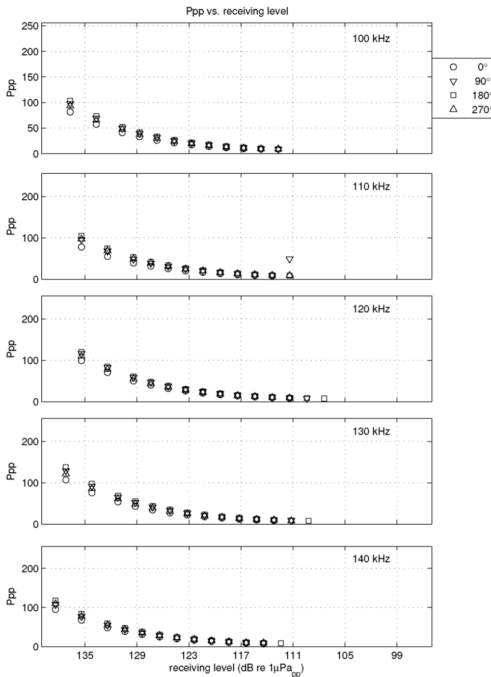
Figure II-5 Calibration results: Ppp vs frequency (this page) and Ppp vs receiving levels (next page) CPOD 862 after deployment.
