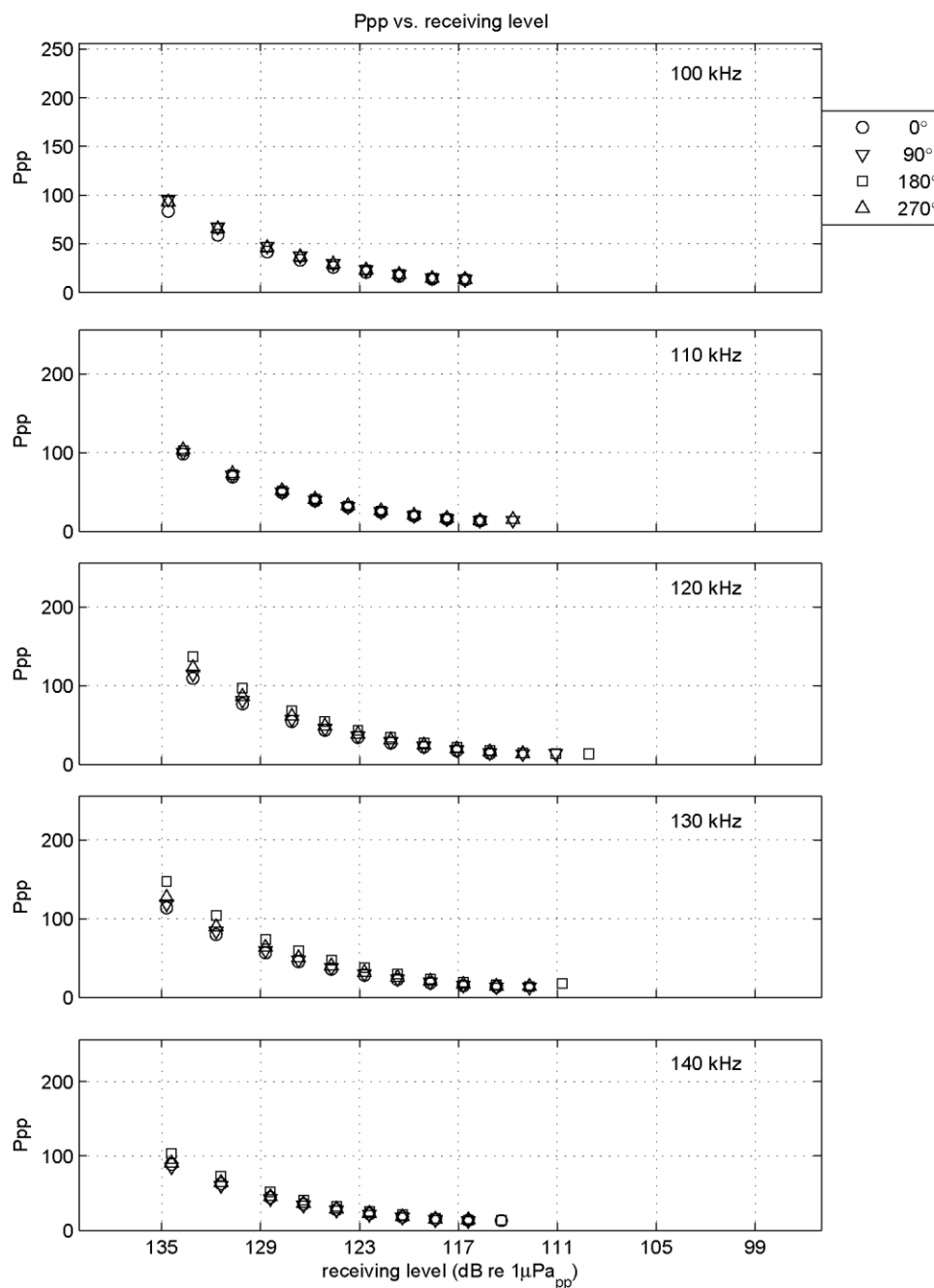
Figure I-1 Calibration results: Ppp vs frequency (this page) and Ppp vs receiving levels (next page) CPOD 376 before deployment.
