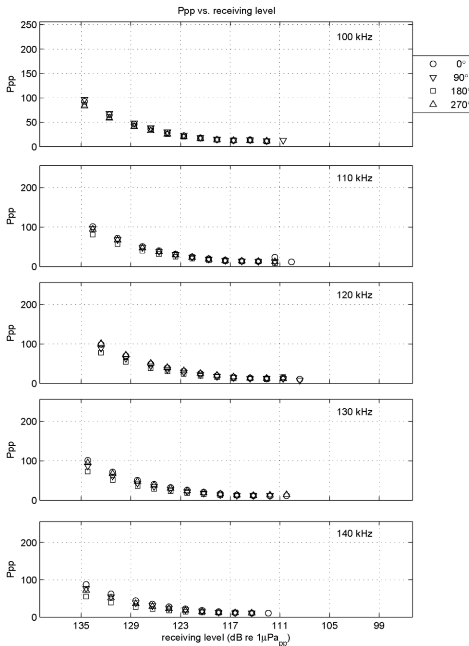
Figure I-13 Calibration results: Ppp vs frequency (this page) and Ppp vs receiving levels (next page) CPOD 1873 before deployment.
