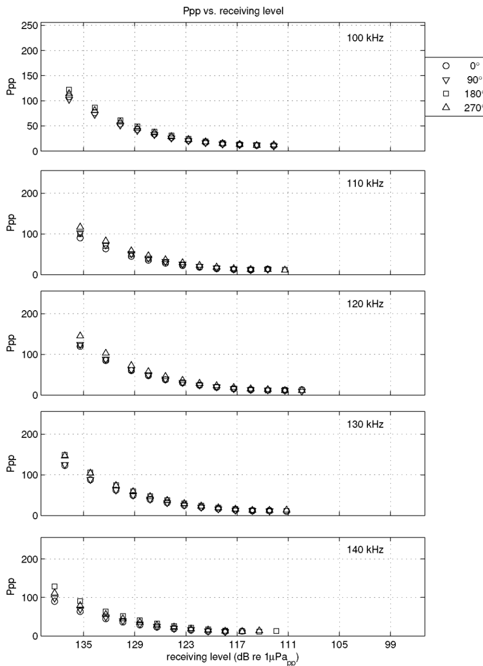
Figure II-8 Calibration results: Ppp vs frequency (this page) and Ppp vs receiving levels (next page) CPOD 1741 after deployment.
