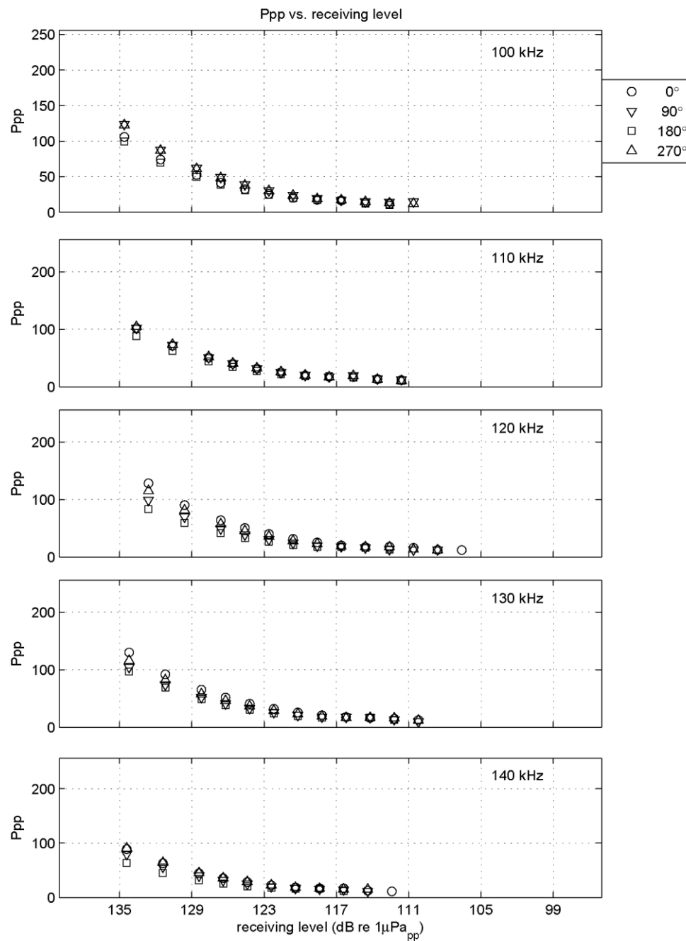
Figure I-16 Calibration results: Ppp vs frequency (this page) and Ppp vs receiving levels (next page) CPOD 1882 before deployment.
