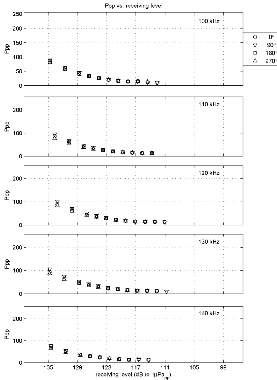
Figure I-19 Calibration results: Ppp vs frequency (this page) and Ppp vs receiving levels (next page) CPOD 3165 before deployment.
