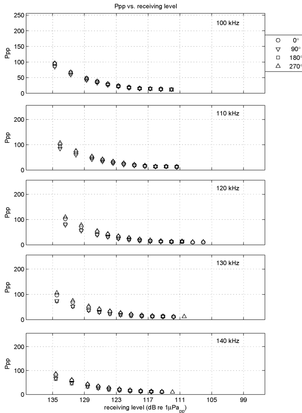
Figure I-15 Calibration results: Ppp vs frequency (this page) and Ppp vs receiving levels (next page) CPOD 1878 before deployment.
