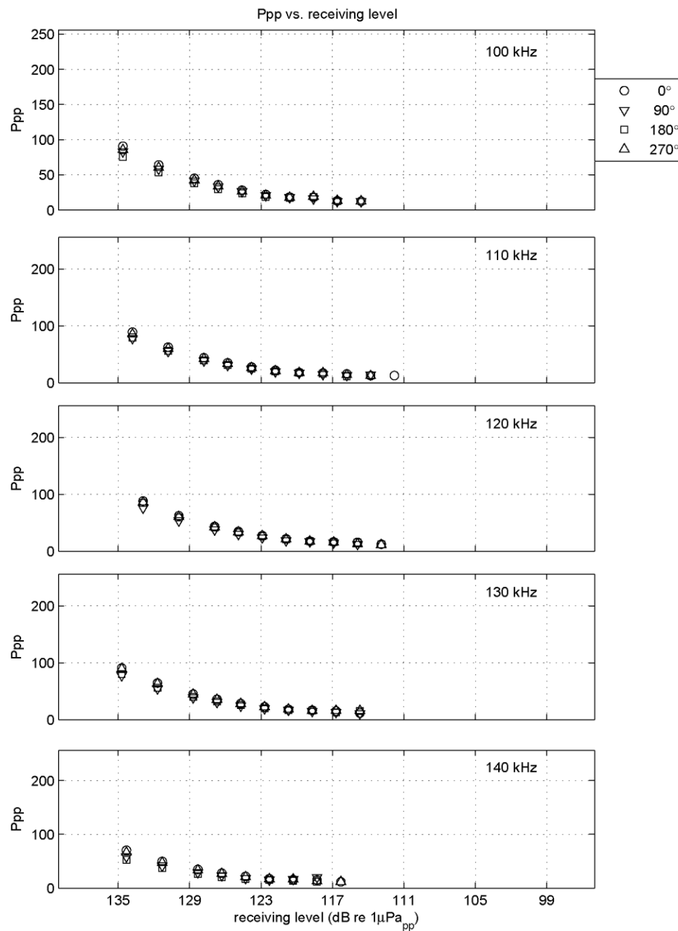
Figure I-20 Calibration results: Ppp vs frequency (this page) and Ppp vs receiving levels (next page) CPOD 3173 before deployment.
