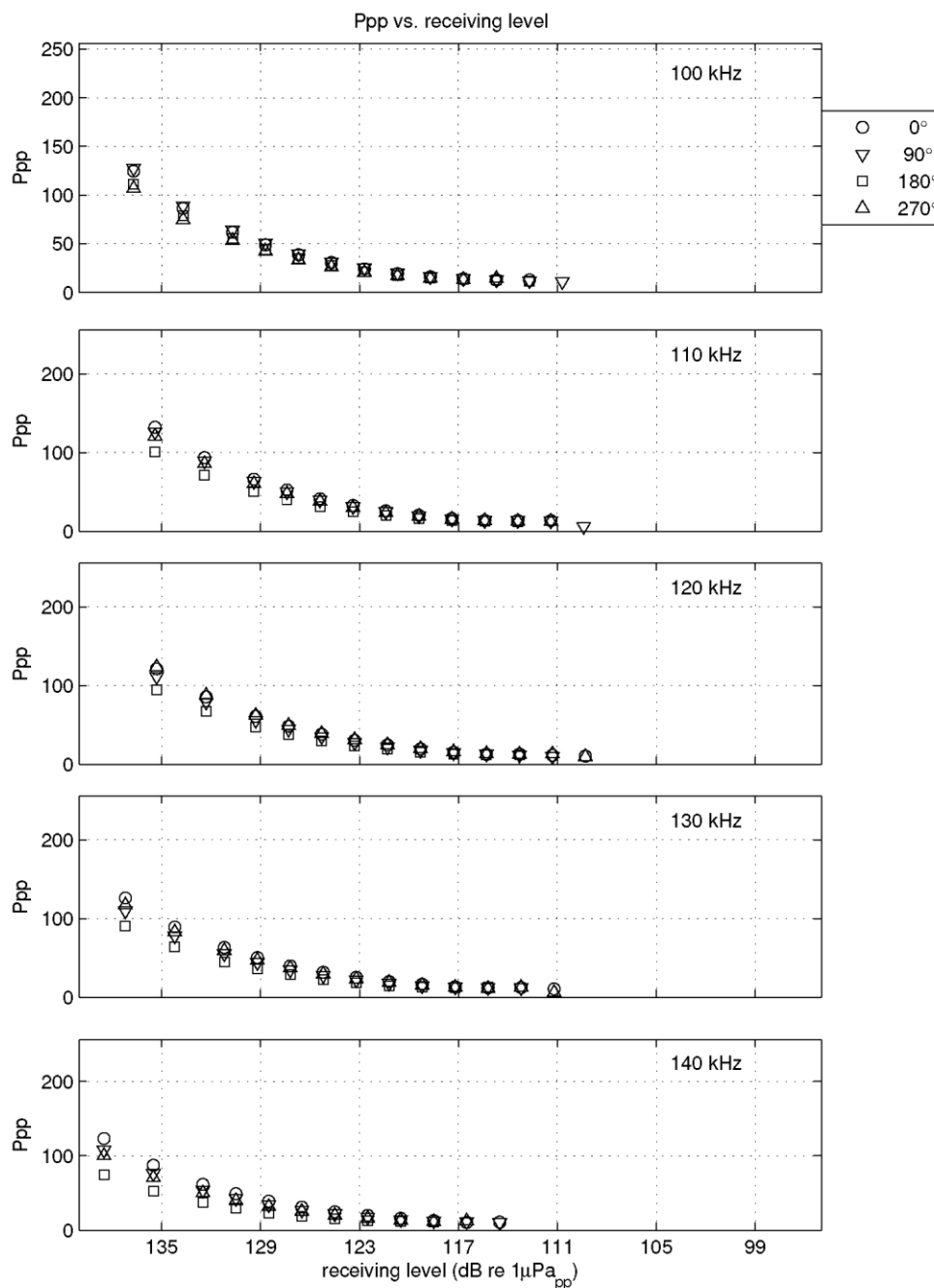
Figure II-15 Calibration results: Ppp vs frequency (this page) and Ppp vs receiving levels (next page) CPOD 1873 after deployment.
