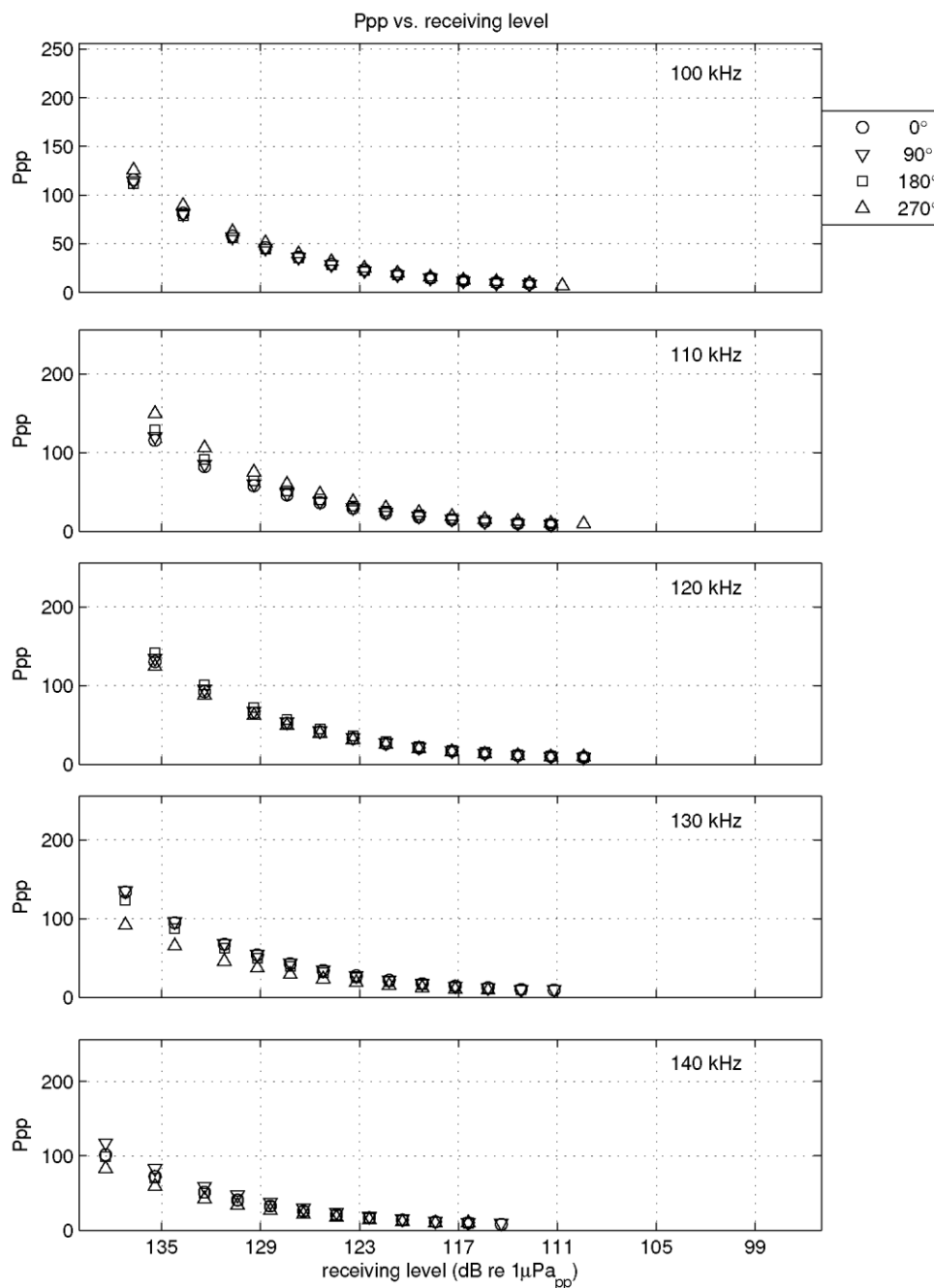
Figure II-16 Calibration results: Ppp vs frequency (this page) and Ppp vs receiving levels (next page) CPOD 1876 after deployment.
