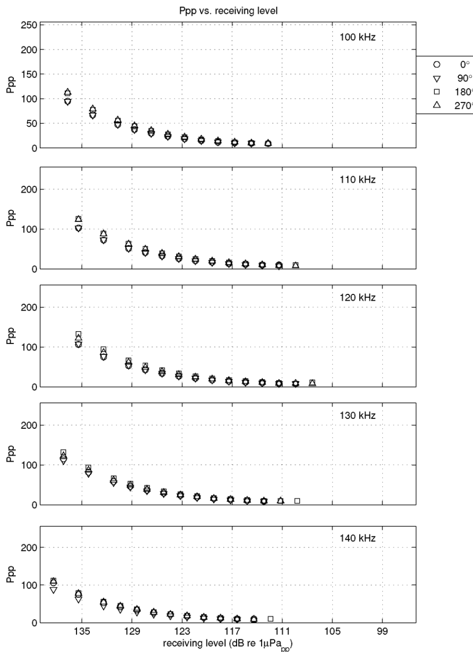
Figure II-13 Calibration results: Ppp vs frequency (this page) and Ppp vs receiving levels (next page) CPOD 1859 after deployment.
