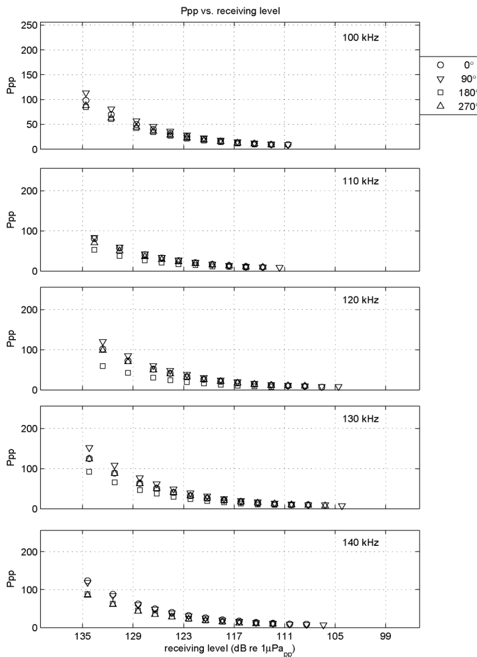
Figure I-9 Calibration results: Ppp vs frequency (this page) and Ppp vs receiving levels (next page) CPOD 1752 before deployment.
