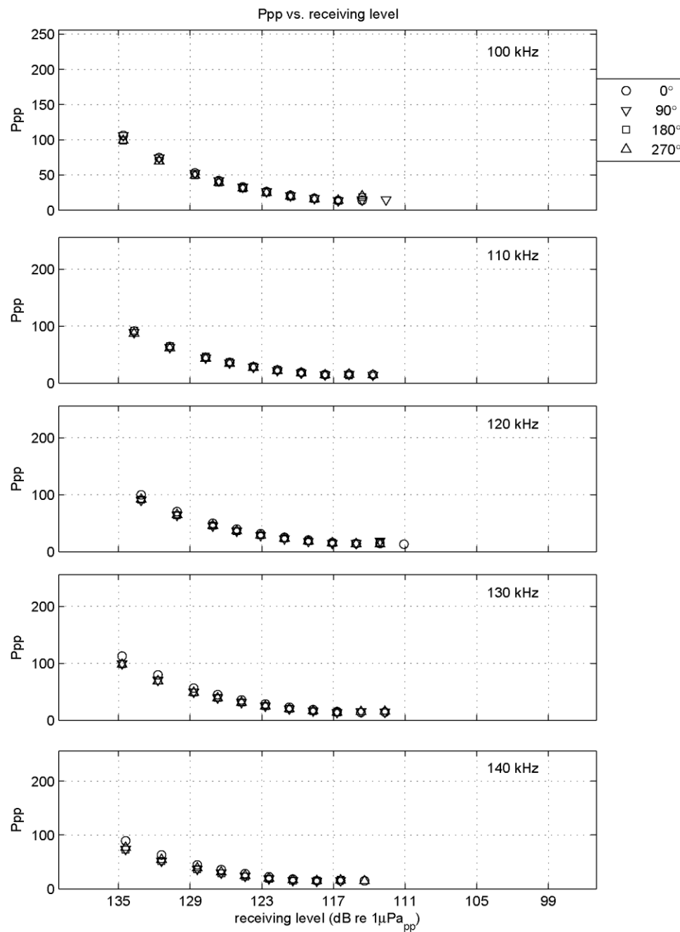
Figure I-4 Calibration results: Ppp vs frequency (this page) and Ppp vs receiving levels (next page) CPOD 395 before deployment.
