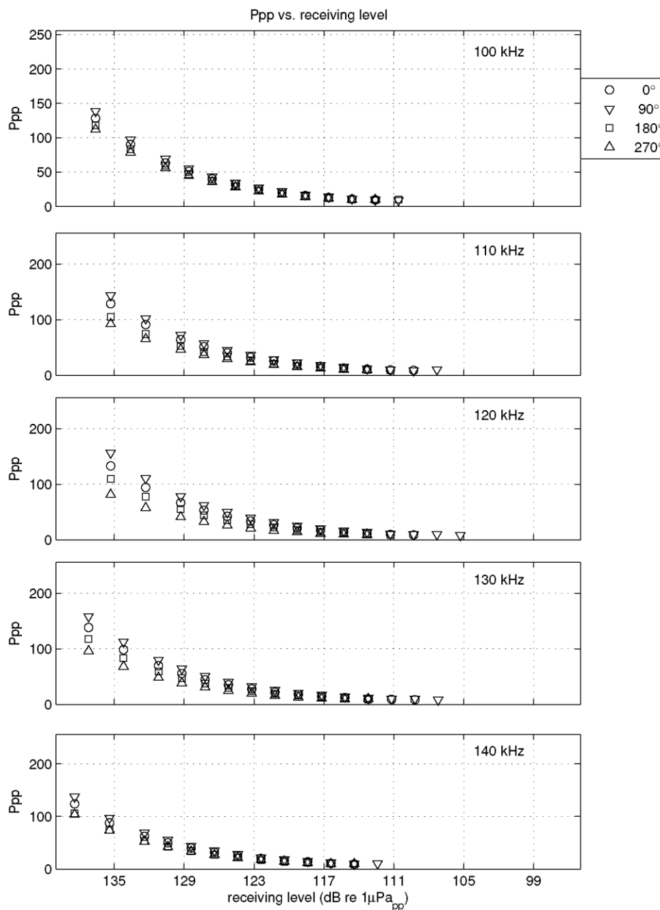
Figure II-12 Calibration results: Ppp vs frequency (this page) and Ppp vs receiving levels (next page) CPOD 1760 after deployment.
