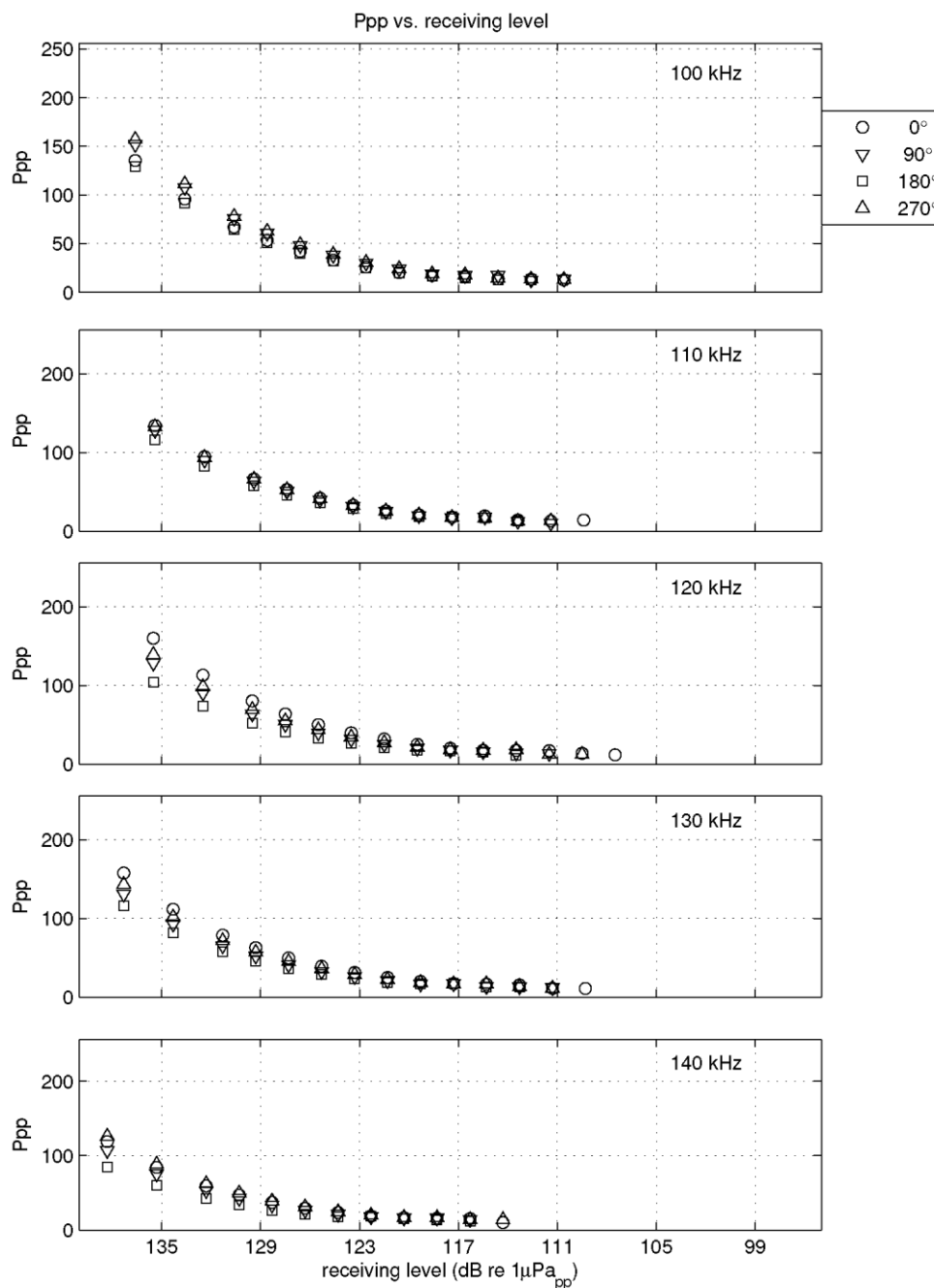
Figure II-18 Calibration results: Ppp vs frequency (this page) and Ppp vs receiving levels (next page) CPOD 1882 after deployment.
