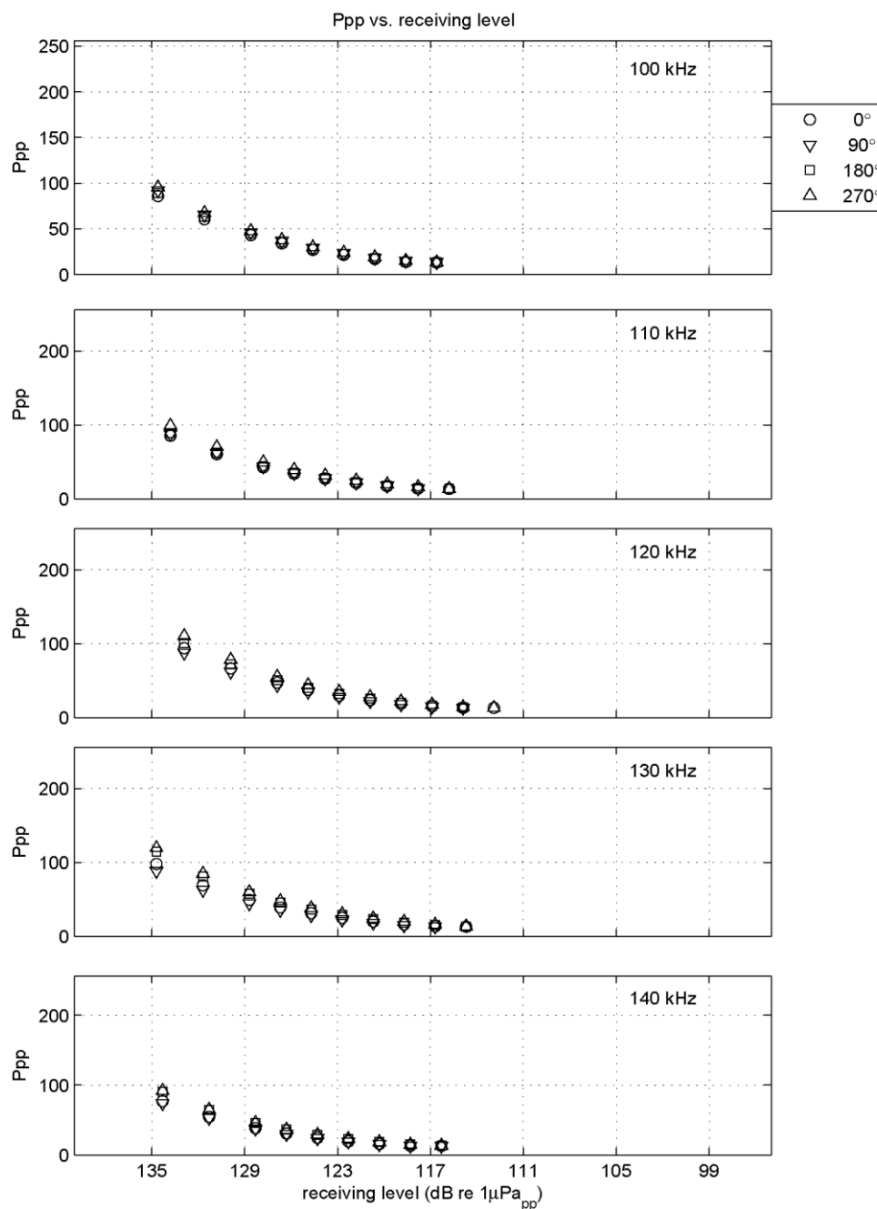
Figure I-3 Calibration results: Ppp vs frequency (this page) and Ppp vs receiving levels (next page) CPOD394 before deployment.
