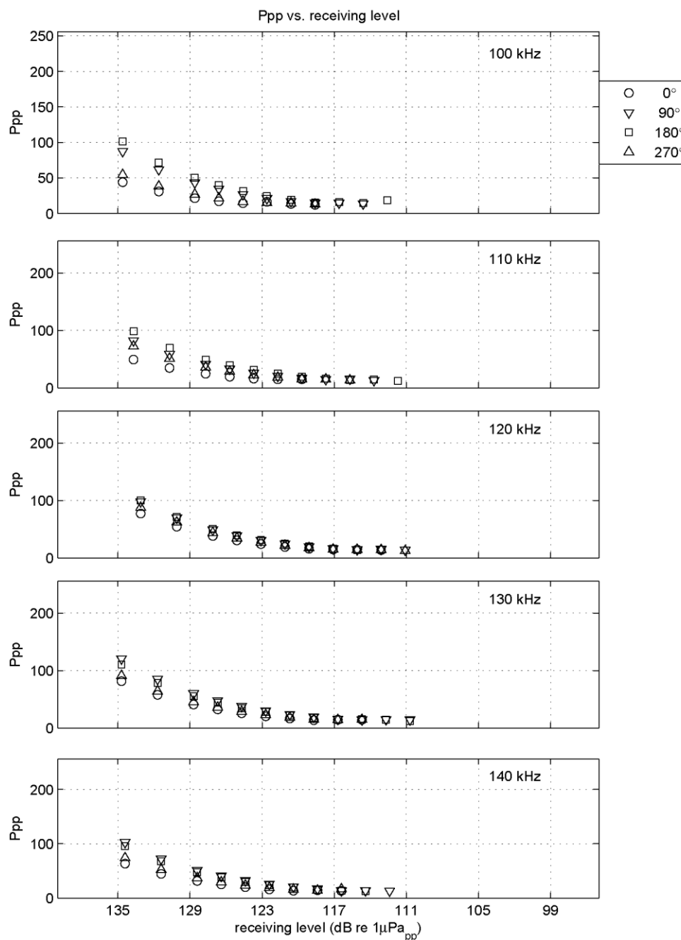
Figure I-6 Calibration results: Ppp vs frequency (this page) and Ppp vs receiving levels (next page) CPOD 1482 before deployment.
