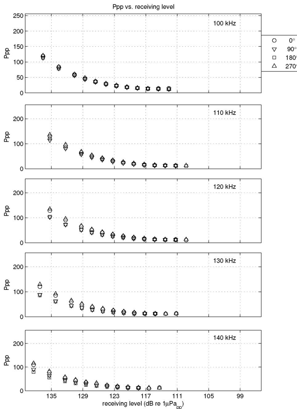
Figure II-17 Calibration results: Ppp vs frequency (this page) and Ppp vs receiving levels (next page) CPOD 1878 after deployment.
