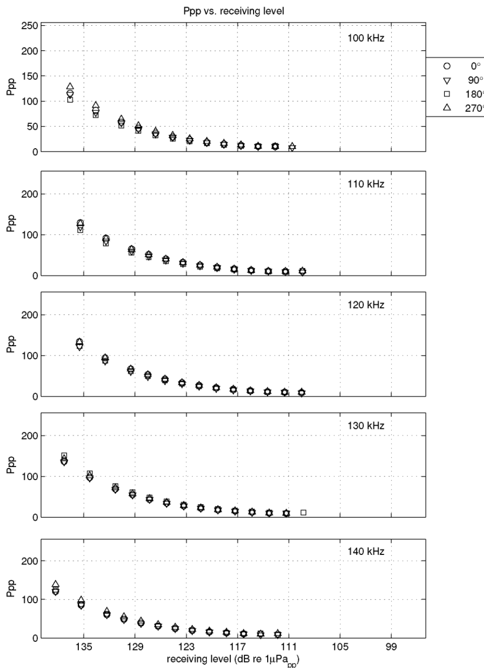
Figure II-19 Calibration results: Ppp vs frequency (this page) and Ppp vs receiving levels (next page) CPOD 1884 after deployment.
