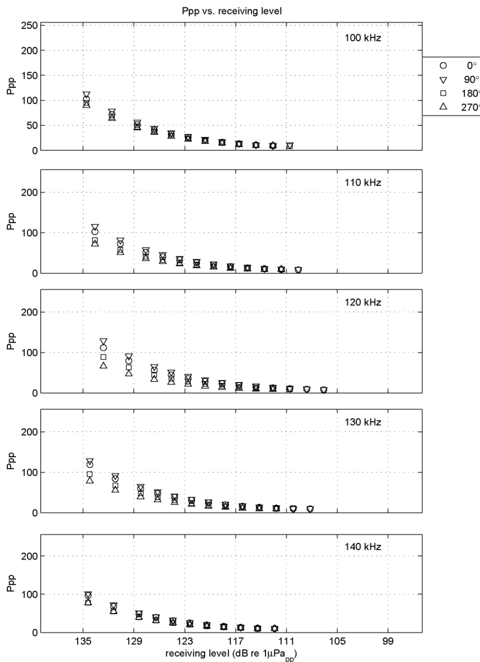
Figure I-10 Calibration results: Ppp vs frequency (this page) and Ppp vs receiving levels (next page) CPOD 1760 before deployment.
