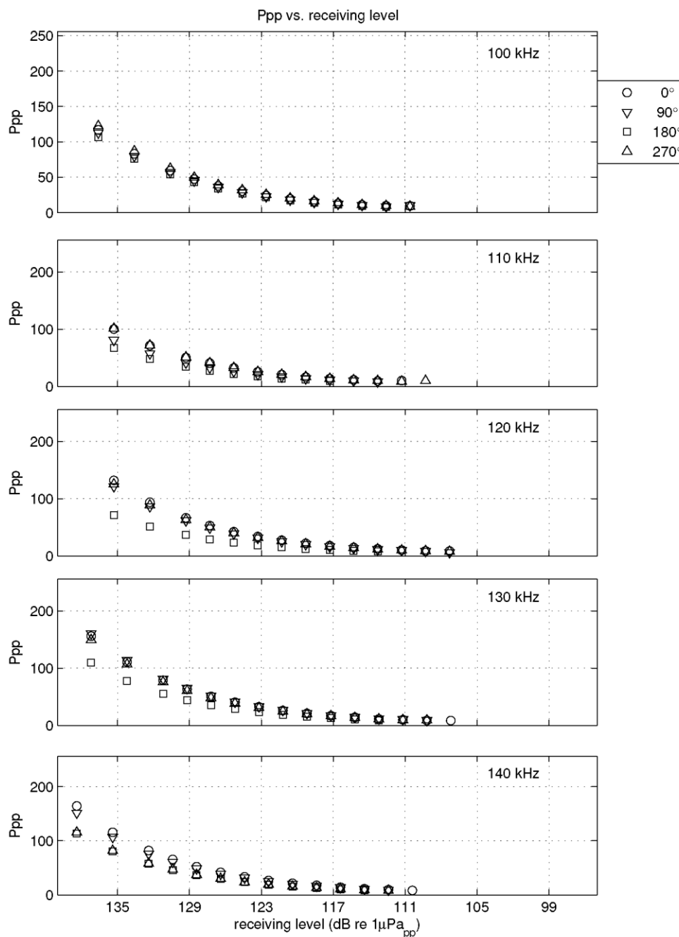
Figure II-11 Calibration results: Ppp vs frequency (this page) and Ppp vs receiving levels (next page) CPOD 1752 after deployment.
