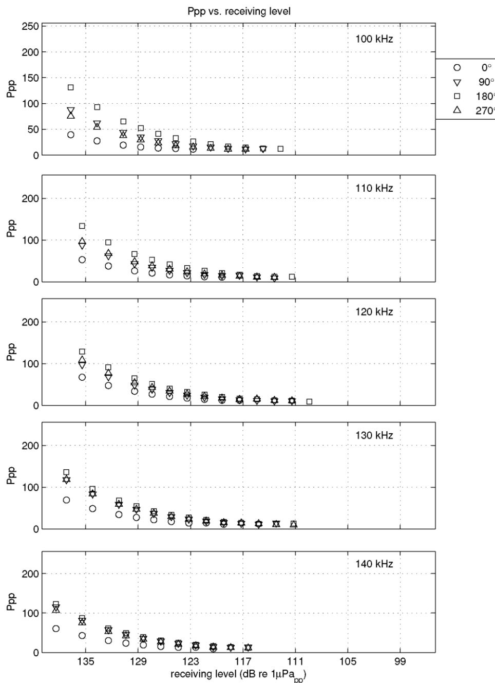
Figure II-6 Calibration results: Ppp vs frequency (this page) and Ppp vs receiving levels (next page) CPOD 1482 after deployment.
