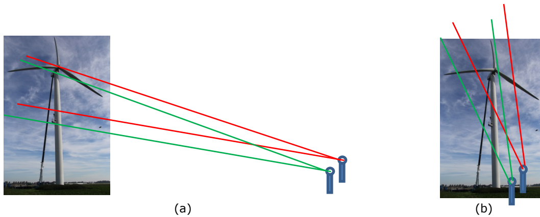
Figure 5: Stereo setup. (a) shows the horizontal stereo setup where the two cameras are placed 80m from the wind turbine facing towards the wind turbine. (b) shows the vertical stereo setup where the two cameras are placed near the wind turbine and facing upwards along the wind turbine.
