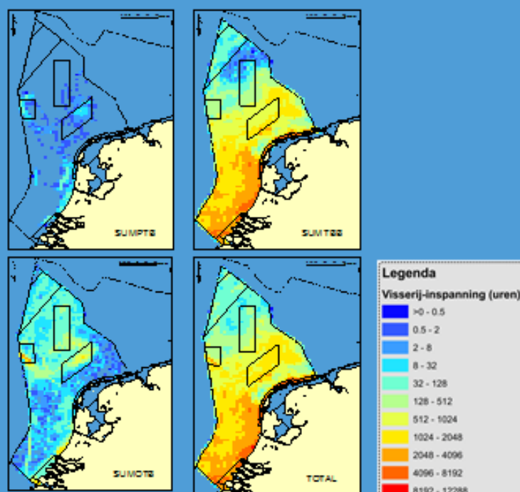
Fig. 11 Fishery effort
