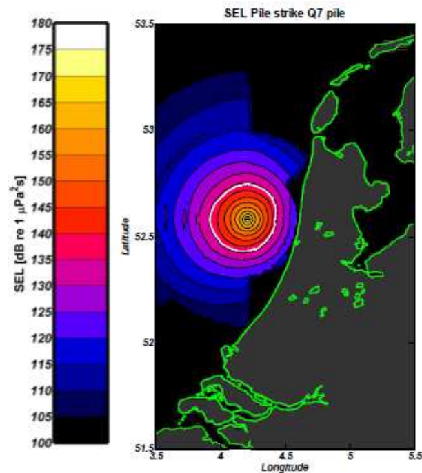
Figure 5 : Unweighted SEL at 1m above the bottom due to a typical hammer strike on a pile in the North sea. A contour of \text{SEL}_1 = 136 \text{ dB re } 1 \mu\text{Pa}^2\text{s} contour is plotted in white, to illustrate the area in which, for example, harbour porpoises may be disturbed by the underwater sound (Nijhof et al. 2014).
