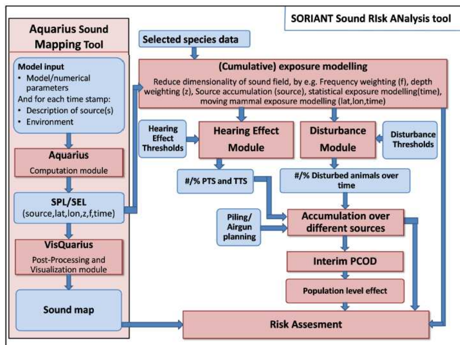
Figure 2 : Implementation of SORIANt framework – modules (red) and interaction between modules. Blue boxes indicate output generated by modules. For a more detailed description of the modules see in Binnerts et al. (2014): source and propagation models (chapter 2) and exposure and assessment modules (chapter 3). Mitigation measures are not yet explicitly modelled (see text for detail).
