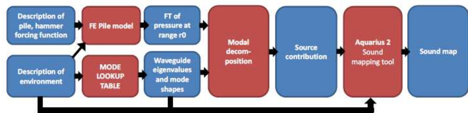
Figure 3 : Schematic picture of coupling FEM source model to the propagation model, used to create sound maps (Nijhof et al. 2014).
