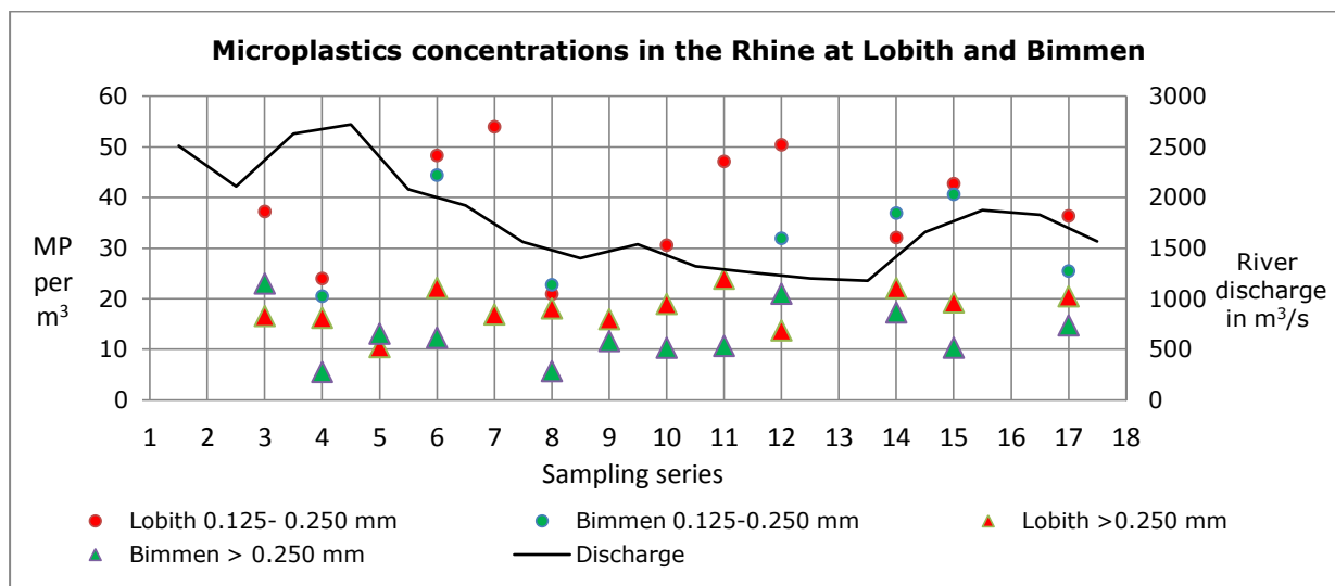
Figure 42. The observed MP particle concentration in the Rhine. The sampling series on the X-axis can be read for both Lobith and Bimmen. Green represents Bimmen and red represents Lobith. Triangles represent the large size fraction and dots represent the small size fraction. The river discharge is line plotted along the secondary y-axis to interpret possible variations over time. Sample series 1 and 2 were not divided in size fractions and hence taken out of account. Samples 13 and 16 were not processed.
