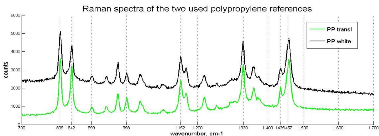
Figure A12. Raman spectra of the two used polypropylene references. The wavenumbers are presented on the X-axis, ranging from 700\text{ cm}^{-1} to 1700\text{ cm}^{-1} (the finger print region). Laser wavelength: 785\text{ }\mu\text{m} . Similarity to isotactic polypropylene was verified with sample spectra from Lobo and Bonilla (2003, pages 236-241) and Shemouratov et al. (2008).
