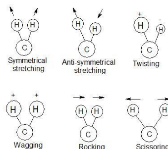
Figure 6. Examples of possible vibrations in a \text{CH}_2 group in a polymer backbone. Figure drawn with Chemschetch.
