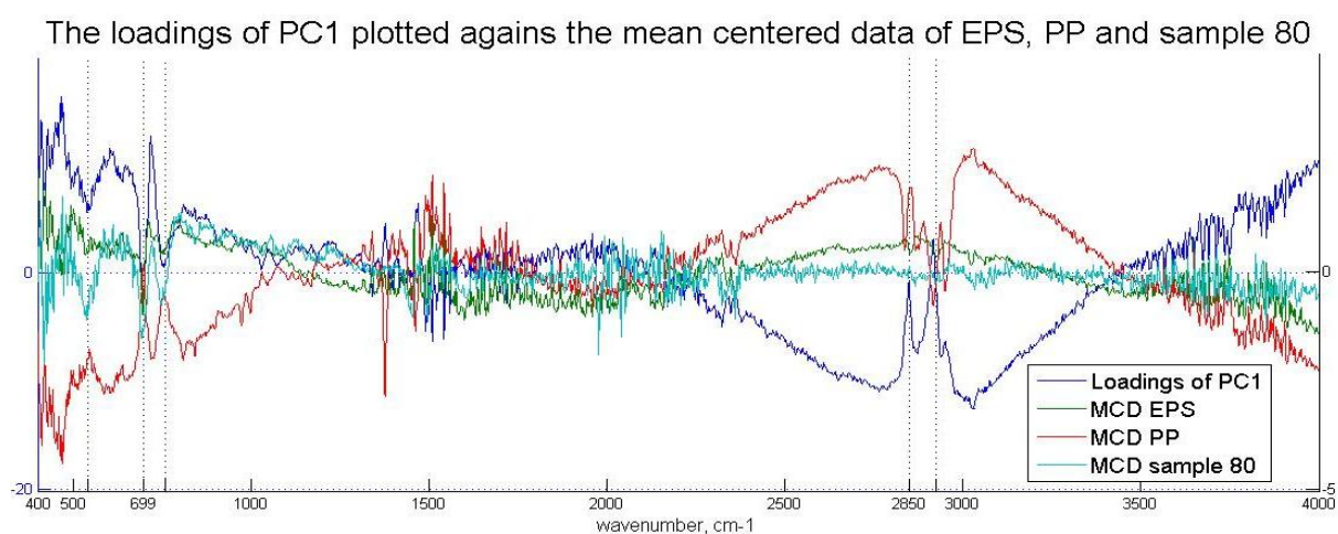
Figure A10. Line plots of the PC1 loadings (blue) versus the mean centered data of the PP reference (red), the mean centered data of the EPS reference (dark green) and the mean centered data of sample 80. The wavenumbers on which PS characteristics are expected, are indicated with the dotted lines. Notice the opposite direction of the PP peak with regard to the loading plot.
