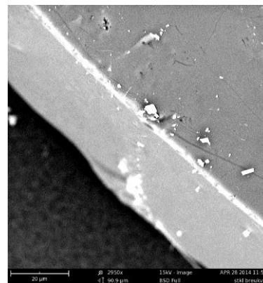
Figure 4. Scanning Electron Microscopic image of the surface (above) and fracture (front) of a coal sheet-like shaped fragment. Scale bar = 20 \mu\text{m}
