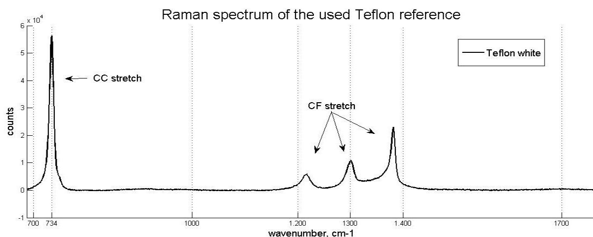
Figure A15. Raman spectrum of the used Teflon reference. Laser wavelength: 785 \mu\text{m} . The wavenumbers are presented on the X-axis, ranging from 700 \text{cm}^{-1} to 1700 \text{cm}^{-1} (the finger print region). Four characteristic peaks are described by Lobo and Bonilla (2003, page 253): three peaks contributed to C-F stretch vibration in between 1200 and 1400 \text{cm}^{-1} and one peak at 734 \text{cm}^{-1} due to skeletal C-C stretching vibrations.
