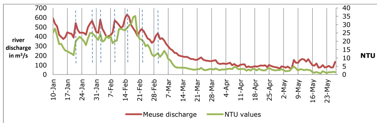
Figure A21. Daily averaged discharge (line plot along the primary Y-axis) and daily averaged NTU values (along the secondary Y-axis) of the river Meuse during the time path of this study.
