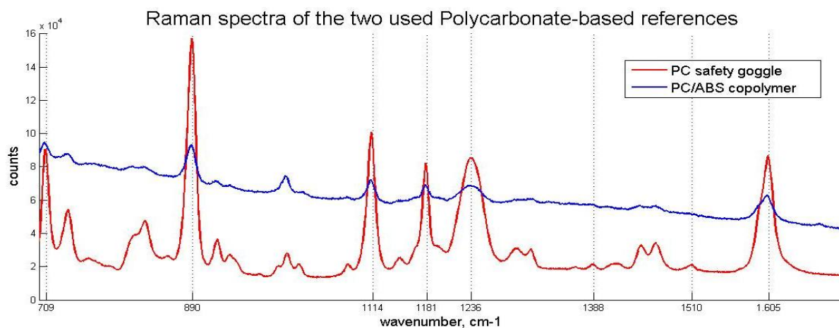
Figure A17. Raman spectra of the two used polycarbonate references. Laser wavelength: 785 nm. The wavenumbers are presented on the X-axis, ranging from 700 cm -1 to 1700 cm -1 (the finger print region). The peak intensity differs, but individual line plots show clear similarity. Influences of ABS in the copolymer were not observed. Similarity to type A bis-phenol polycarbonate, commercially known as Lexan, was verified with Lobo and Bonilla (2003, page 330, fig. RS38).
