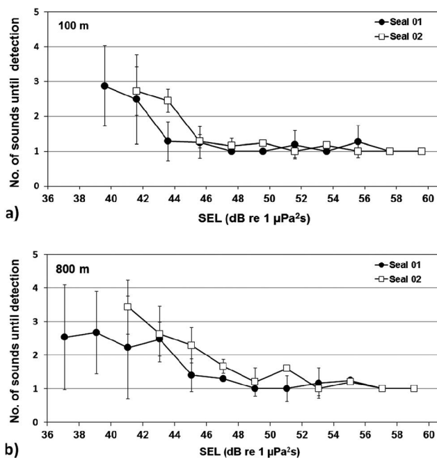
FIG. 4. The received broadband sound exposure level (SEL based on a single pulse) in relation to the mean pile driving sound number (of series of five sounds) which the two harbor seals detected (the bars indicate \pm the standard deviation, sample sizes vary between 2 and 41 due to the up-down hearing test method used); (a) for sounds recorded at 100 m from the pile driving location, and (b) for sounds recorded at 800 m. For SPL (dB re 1 \mu\text{Pa} ), add 9 dB to the SEL values.
