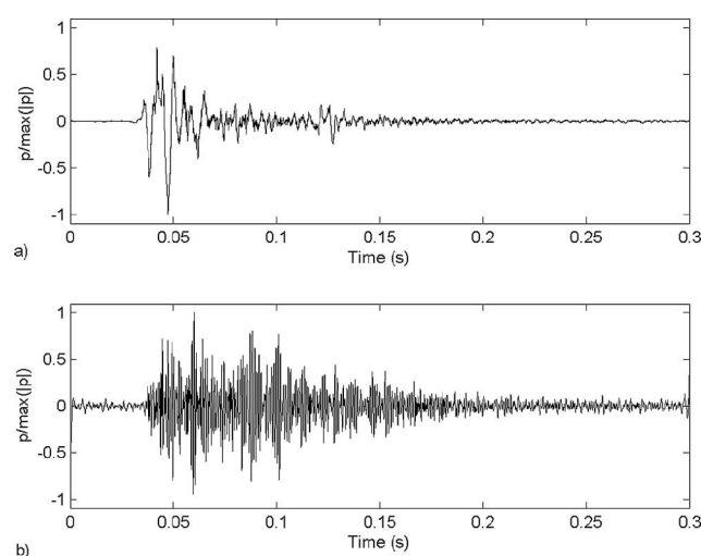
FIG. 1. Waveform (a) of a single pile driving sound recorded at 100 m from the pile driving site and (b) of the played back sound in the pool. The amplitude of the sound pressure is scaled to the maximum absolute value of instantaneous sound pressure.
