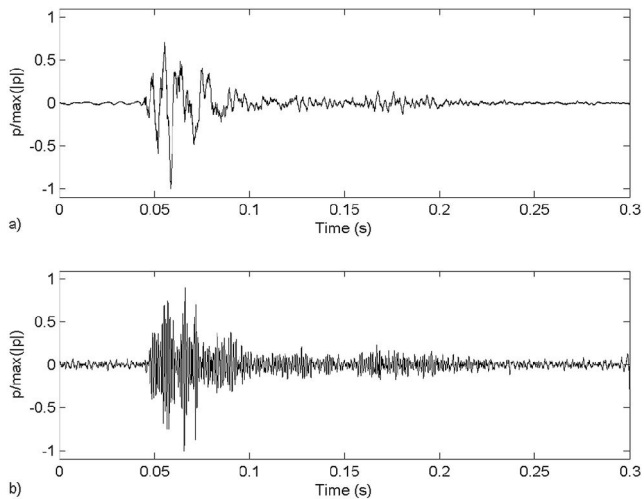
FIG. 2. Waveform (a) of a single pile driving sound recorded at 800 m from the pile driving site and (b) of the played back sound in the pool. The amplitude of the sound pressure is scaled to the maximum absolute value of instantaneous sound pressure.
